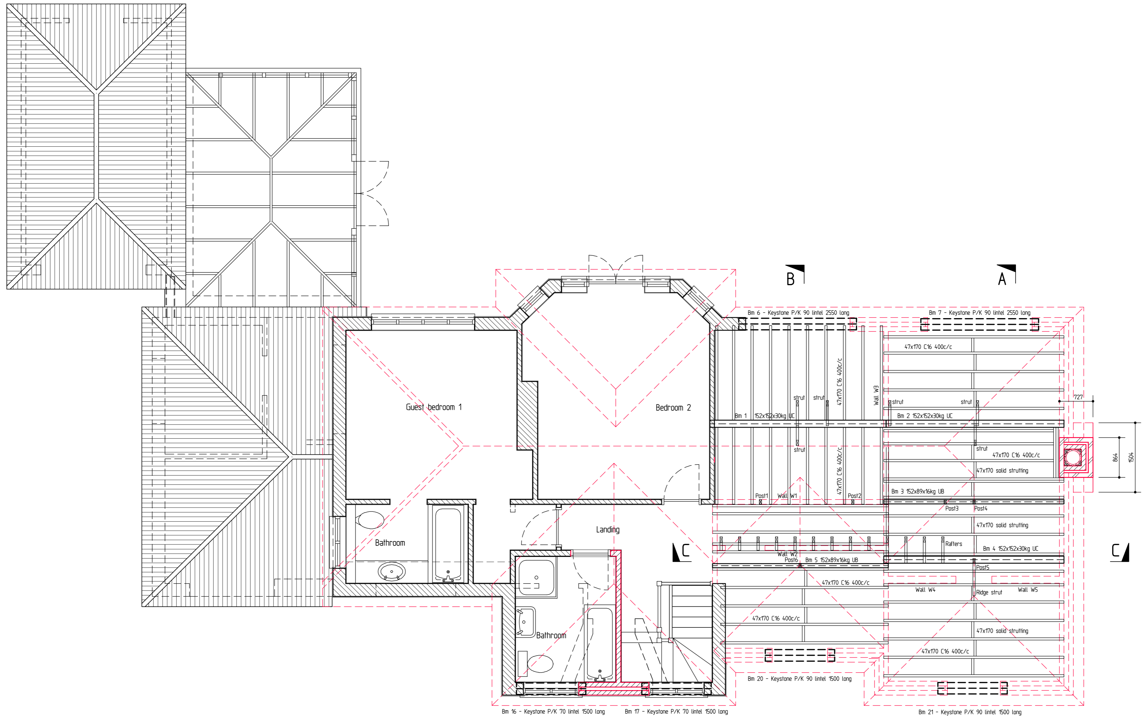
Ceiling Joist Plan Showing supporting walls under
